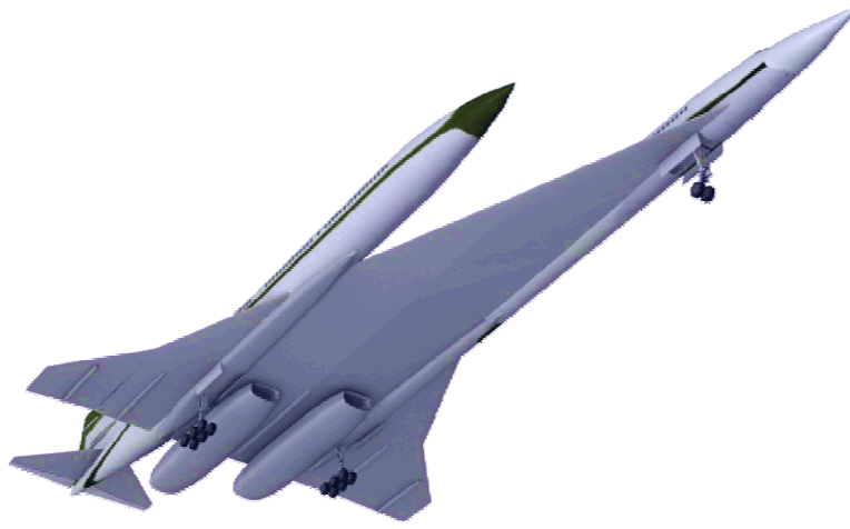
figure 6. Unusual Symmetry - Horizontal Tail
